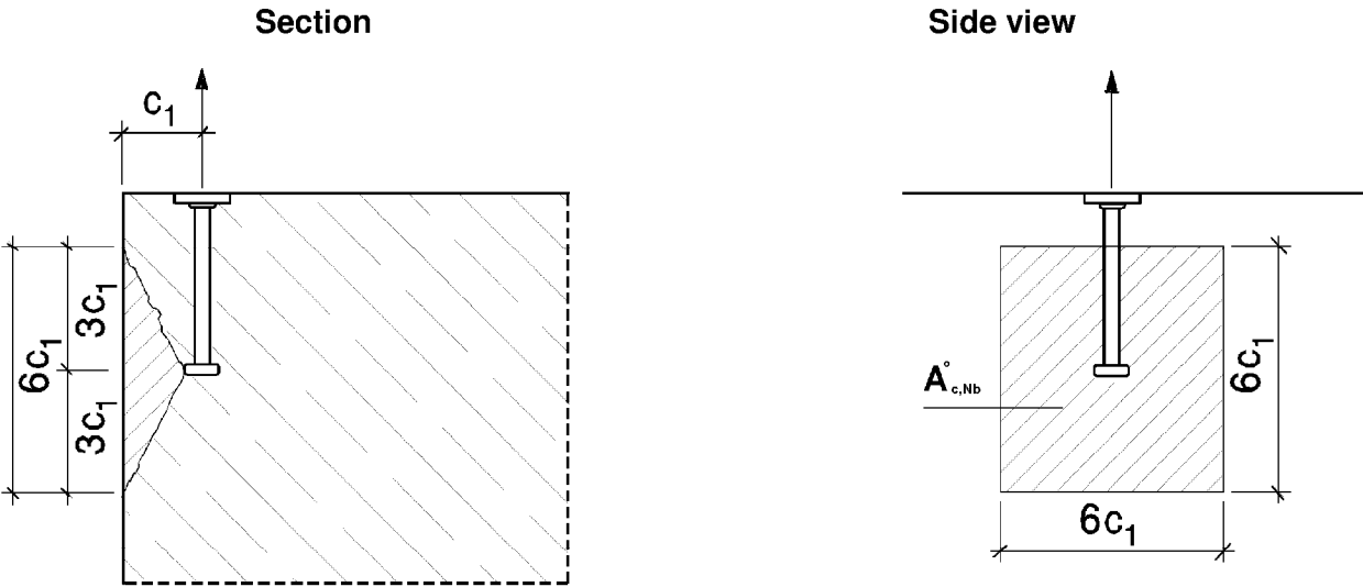
Figure 3: Idealized concrete cone of the headed stud in the case of local concrete blow-out failure at the edge of an individual headed stud
