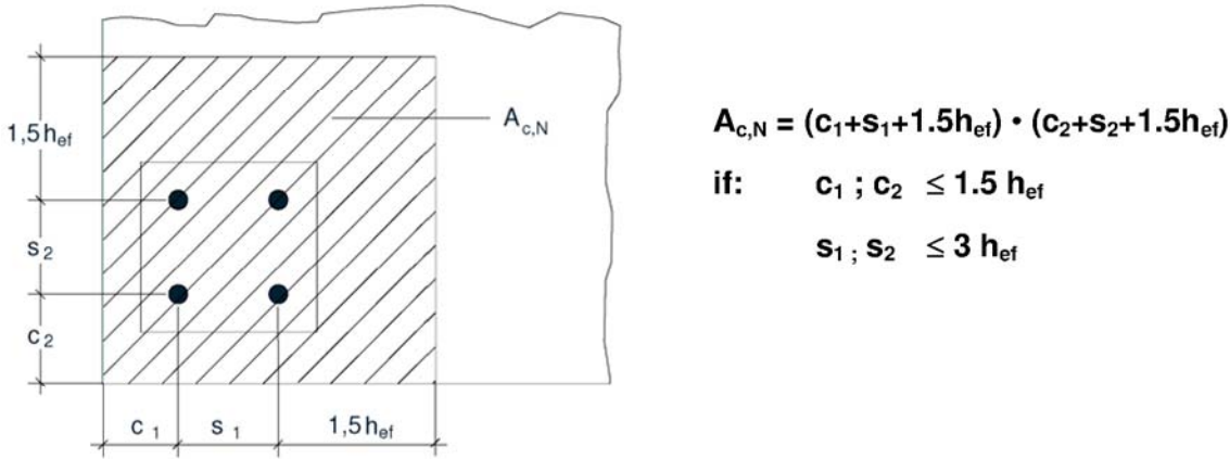
Figure 2: Example of actual areas A_{c,N} of the idealized concrete cones of headed stud in the case of axial tension load
