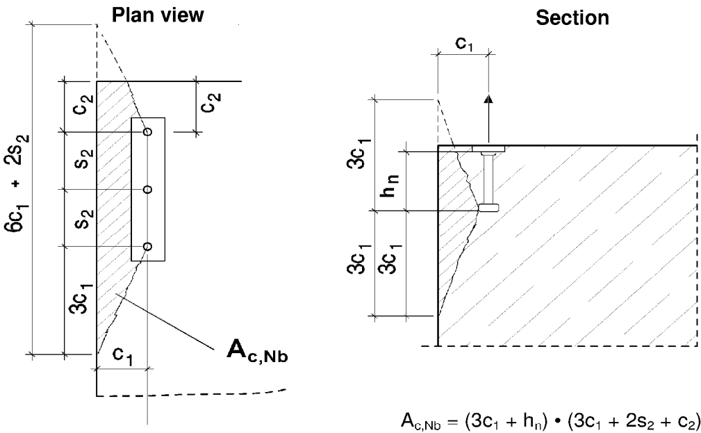
Figure 3: Idealized concrete cone of the headed stud in the case of local concrete blow-out failure at the edge of an individual headed stud
