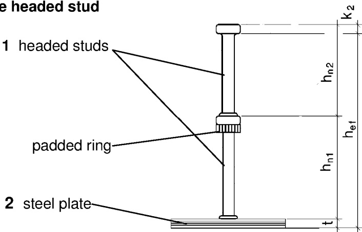
Fig. 2: Double headed stud
